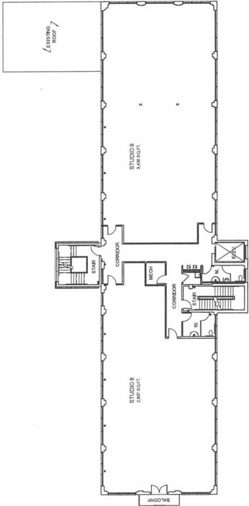
I THIRD FLOOR PLAN SCALE: 1/8" = 1'-0"
